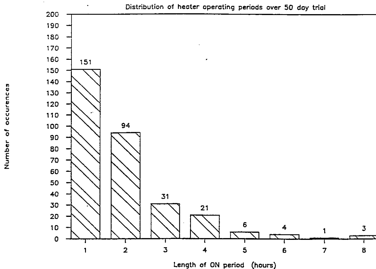
Fig. 13. Pseudo-random heating sequences: 5-day sample and 50-day distribution
