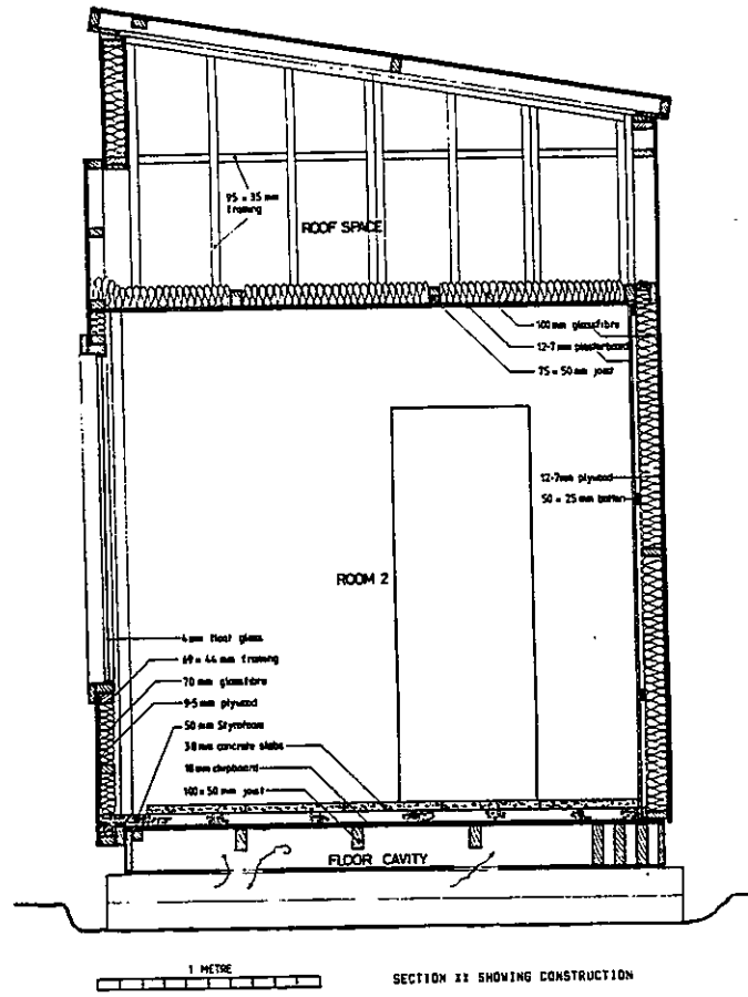
Fig. 11. Construction Details of the EMC Test Rooms
