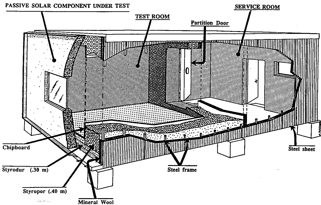
Fig. 8. Sketch of the PASSYS test cell
