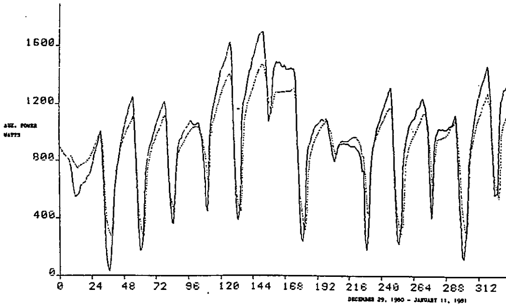
Heating power.
