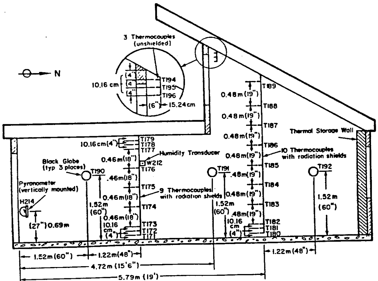
Fig. 15. Longitudinal section and air temperature sensors in the direct gain cell 4
