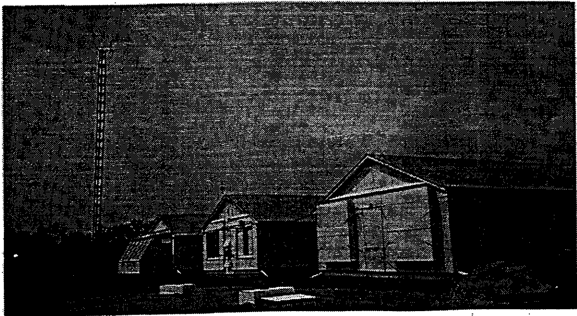
Plate 2. The Canadian Direct Gain Building photographed in 1985
