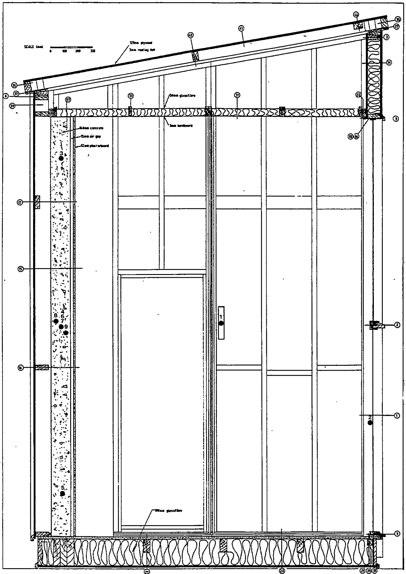
Fig. 2. Vertical cross-section through Cell 1 looking east
