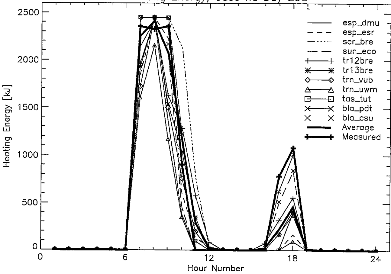
Heating Energy, Case hd Day 298
