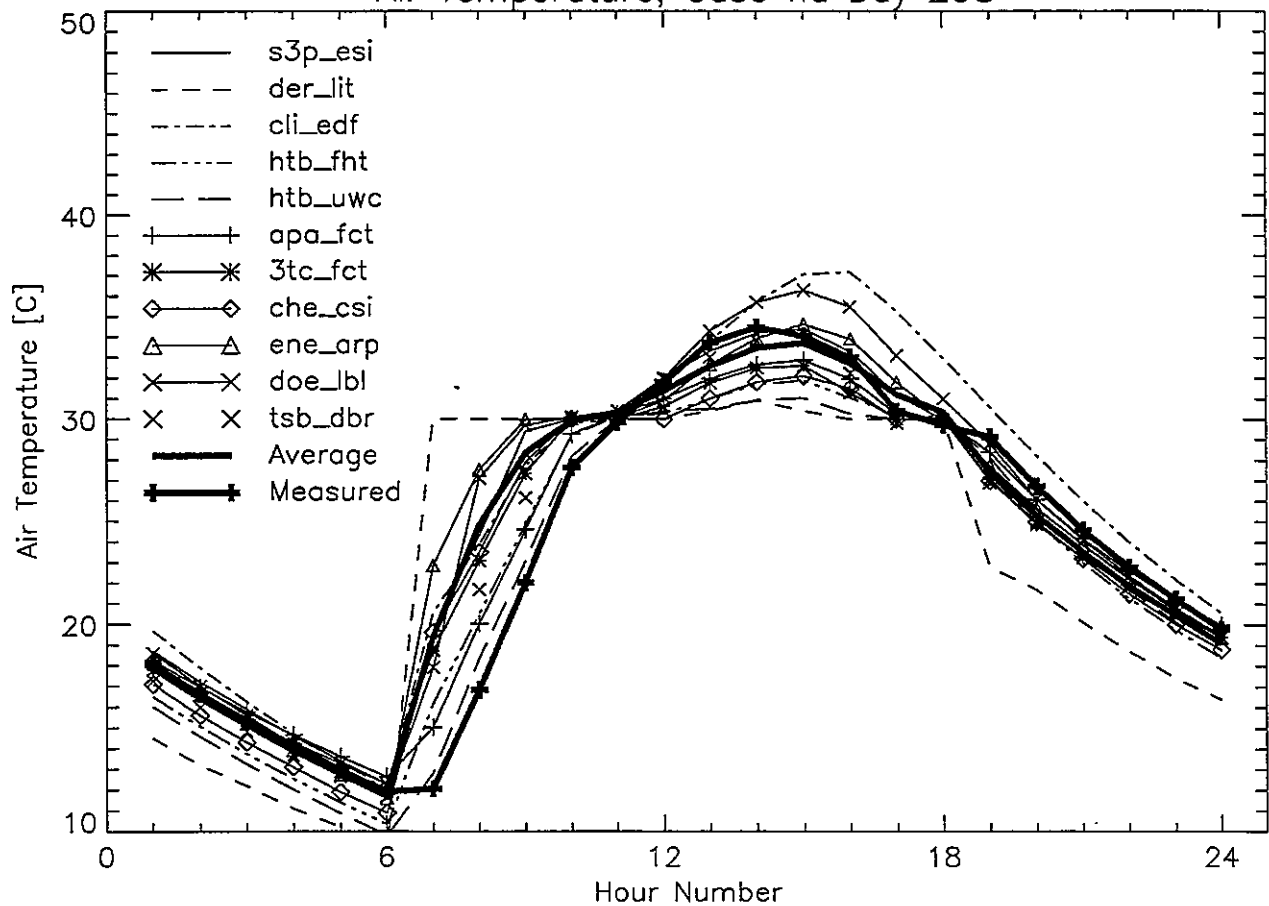
Air Temperature, Case hd Day 298
